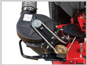
TURBO-Pro Blower* — Length: 31" Height: 16.5" Width: 19" Approximate blower weight: 50 lbs. (44"/48") / 53 lbs. (52") / 55 lbs. (61"), includes mounting bracket
