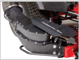
TURBO-Pro Max Blower* — Length: 36" Height: 18" Width: 21" Approximate blower weight: 72 lbs. (52") / 64 lbs. (61"), includes mounting bracket
